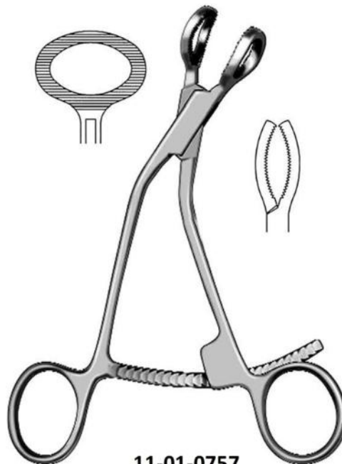
11-01-0757 Bishop Bone Holding Forceps 23 cm / 9"
