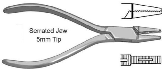
11-01-0405 Flat Nose Pliers 14 cm / 5 1/2"
