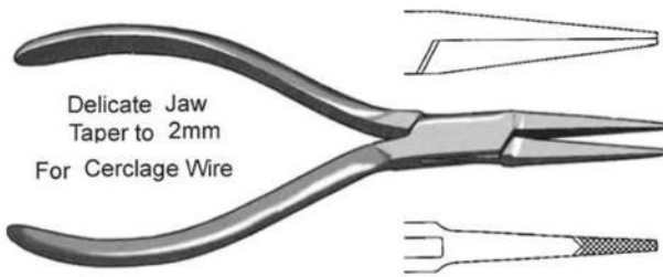
11-01-0395 Flat Nose Pliers 15 cm / 6"
